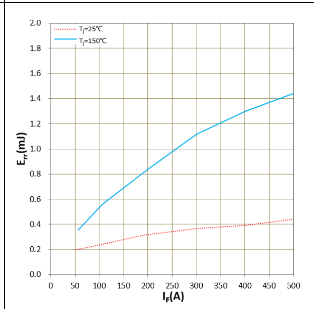
Figure 19. E_{rr} vs I_F V_{DD} = 600\text{V} , R_G = 4.5\Omega , V_{GS} = +15\text{V}/-4\text{V} Inductive Load
